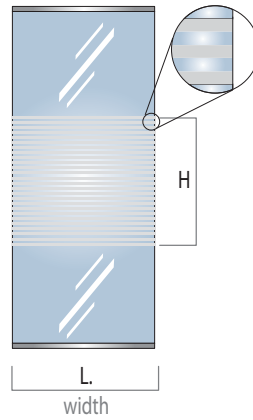
TYPE 2 (passo 20mm) SATINATURA MILLERIGHE SATIN STRIPED-EFFECT SATIN MILLERAIES
